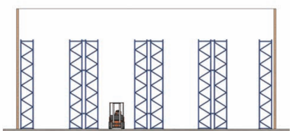
The most common conventional system made up of a single-entry rack fitted to the wall and double-entry racks in the middle.
